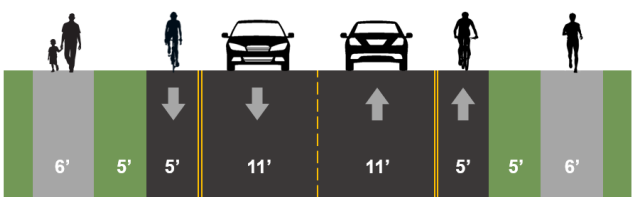
Minor Collector – 70' ROW
