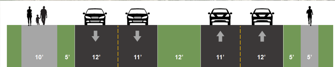
Minor Arterial – 100' ROW
